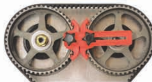
PBT70896 Timing Gear Clamp Used on Twin-cam & Quad-cam Engines Hold Valve Timing During Belt Replacement
